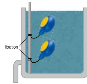
MULTI-LEVEL SWITCHING
