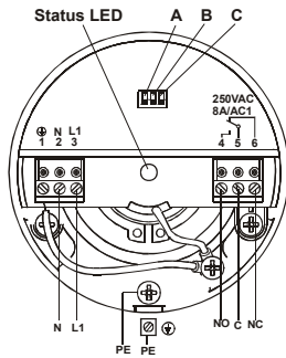
Figure 7. Wiring of relay output version
